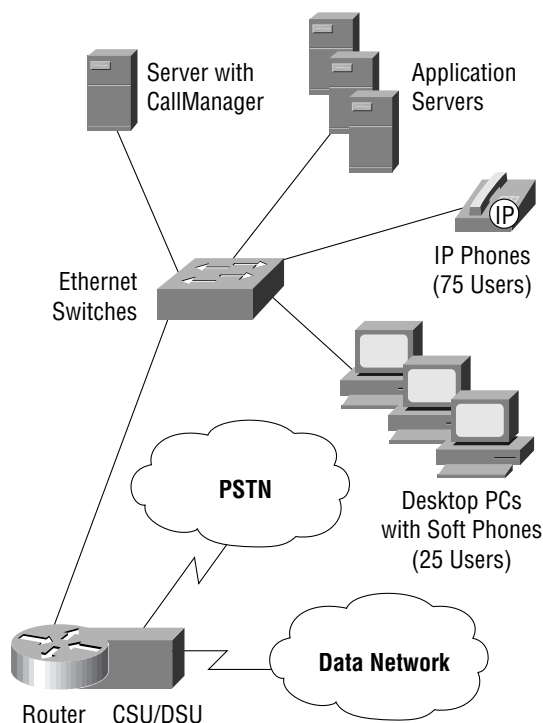
Figure 10 100-User Network—Year 3
