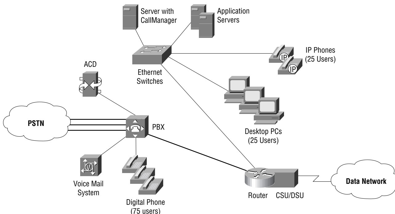
Figure 8 100-User Network—Year 1
