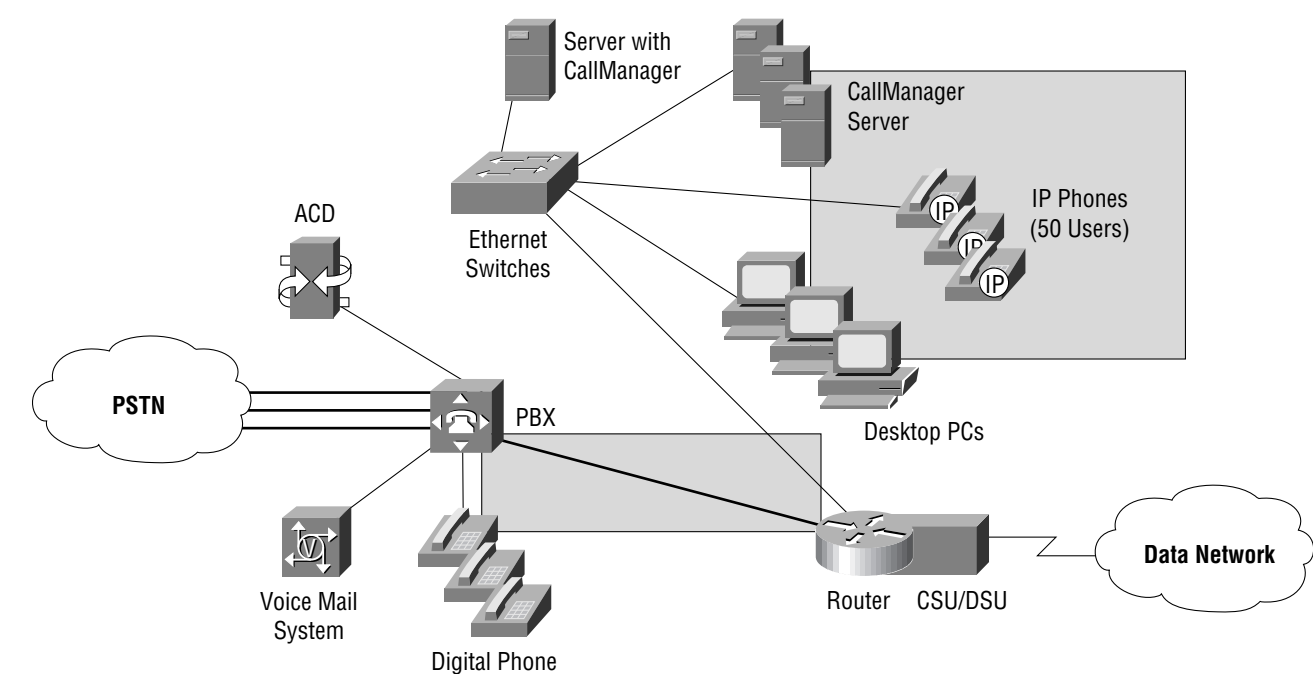
Figure 13 1000-User Network Year-1 Implementation
